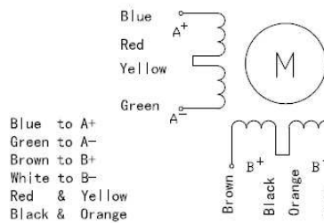
Bipolar (Series) Connection
