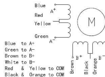
Unipolar Connection
