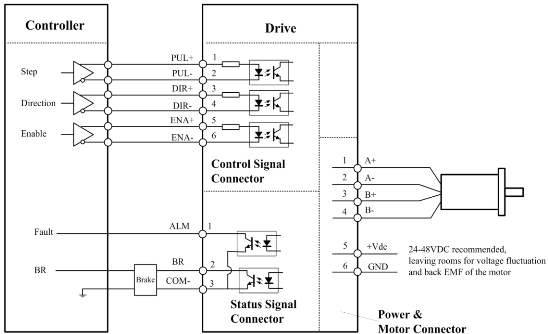
Figure 12 Typical connection
