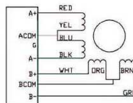
Unipolar Connection
