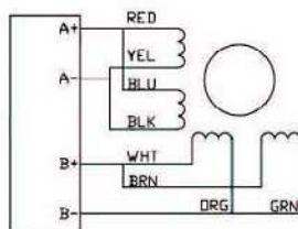
Bipolar (Parallel) Connection
