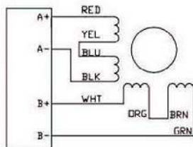
Bipolar (Series) Connection
