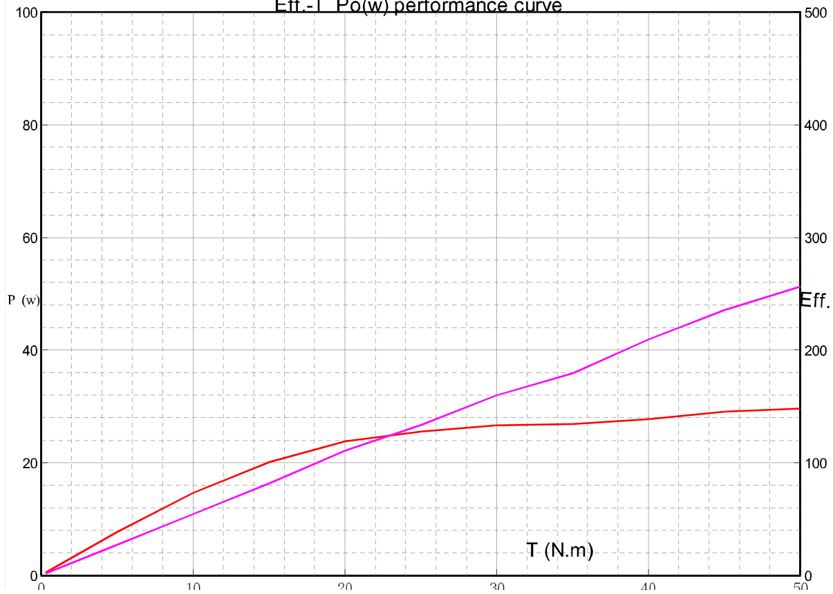
Eff.-T Po(w) performance curve
