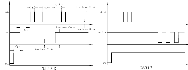
Figure 10: Sequence chart of control signals
