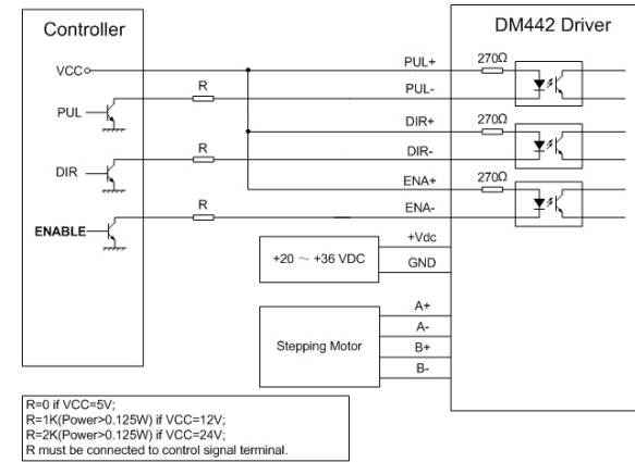
Figure 9: Typical connection
