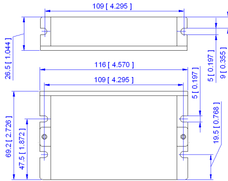
Figure 1: Mechanical specifications
