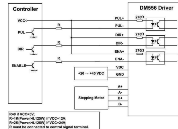
Figure 9: Typical connection
