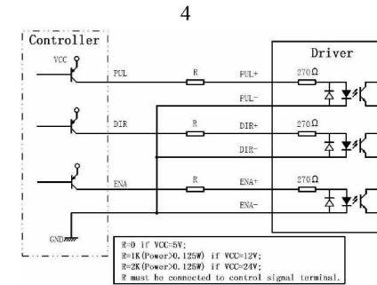
Figure 3: Connection to PNP signal (common-cathode)
